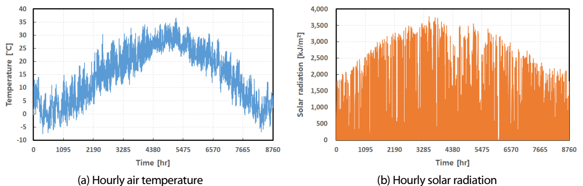
Fig. 1 2017 Weather data in Gwangju
